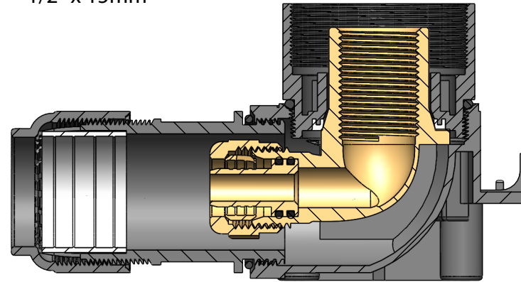
SECTION B-B SCALE 1 : 1.4
