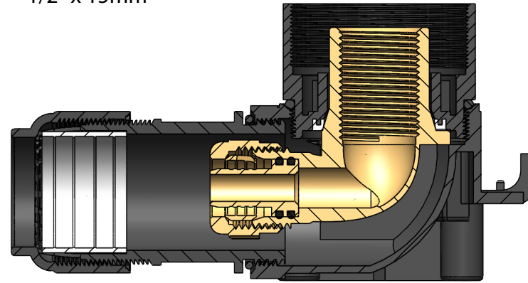
SECTION B-B SCALE 1 : 1.4
